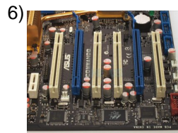
expansion slot
