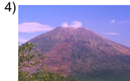
volcano
