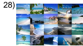
coasts
