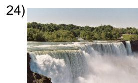
waterfall
